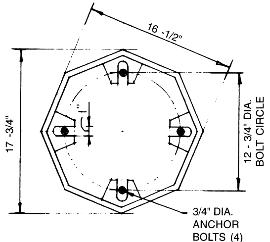
Bolt Circle 12-3/4" DIA. BOTTOM PLAN
