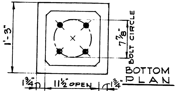
PLAN OF TOP
