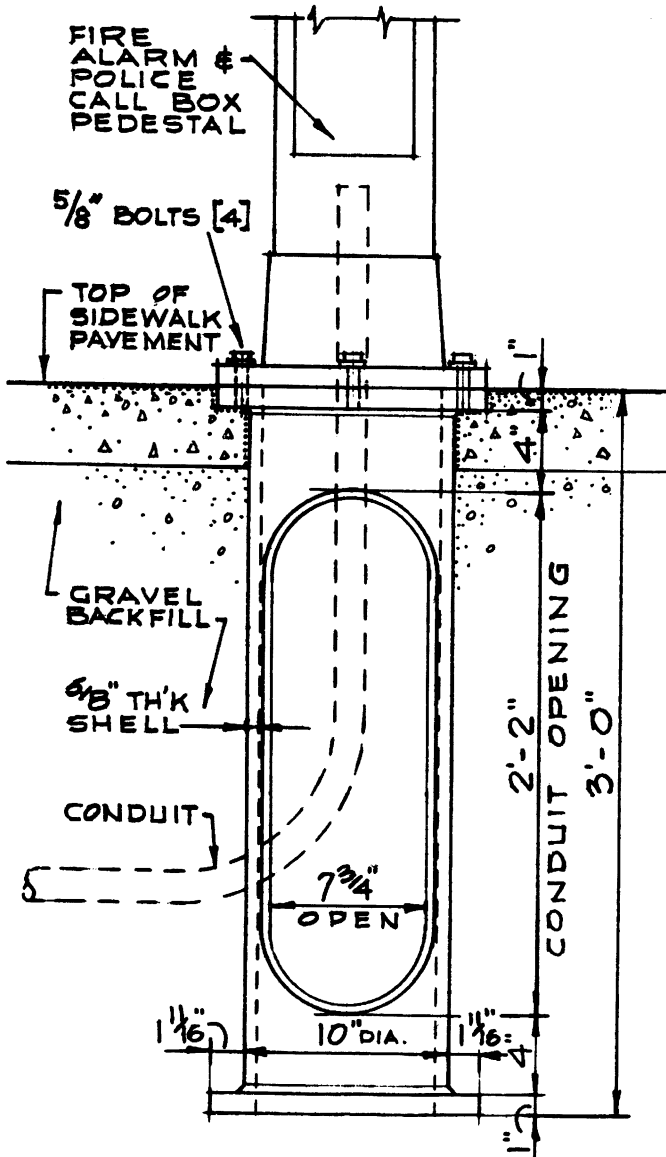
FOUNDATION ELEVATION FOR PEDESTALS
