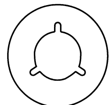
(3) 3/4" ANCHOR BOLTS ON 12 1/4" ± BOLT CIRCLE
