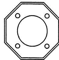
9-1/2" +/- DIA. BOLT CIRCLE FOR 3/4" ANCHOR BOLTS
