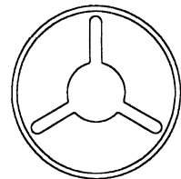
11" +/- DIA. BOLT CIRCLE FOR 3/4" ANCHOR BOLTS
