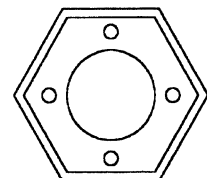
11-1/4" +/- DIA. BOLT CIRCLE FOR 3/4" ANCHOR BOLTS
